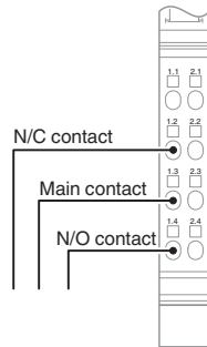
Figure 6 Actuator connection; floating connection
