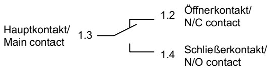
Figure 8 Output relay contacts
